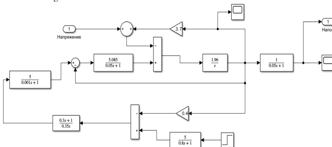
Fig. 2. Mathematical model of a pump
